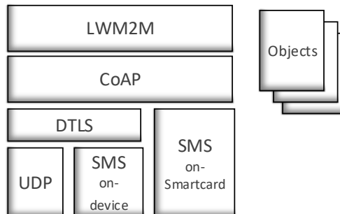
Figure A.5.1-1: LWM2M Protocol Stack
